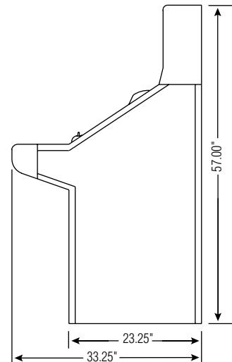
Slant-Top with Standard Top Box
