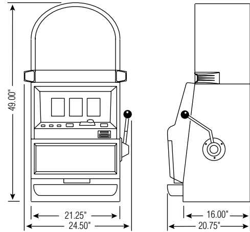
Upright with Round Top Box
